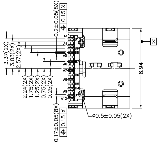
PIN ASSIGNMENT (FRONT VIEW)
