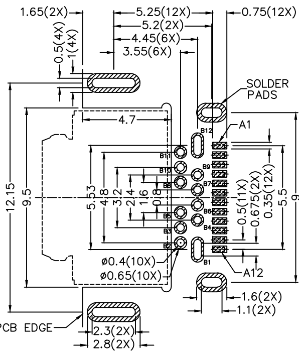
RECOMMENDED PCB LAYOUT TOLERANCE: ±0.05 (TOP VIEW)
