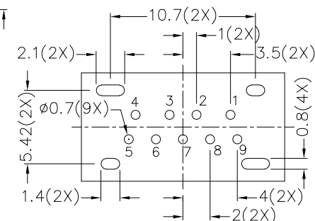
RECOMMENDED PCB LAYOUT TOLERANCE: ±0.05 (TOP VIEW)
